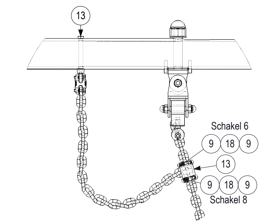
DETAIL C SCALE 1 : 5
