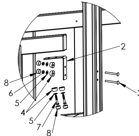
DETAIL C SCALE 1 : 15
