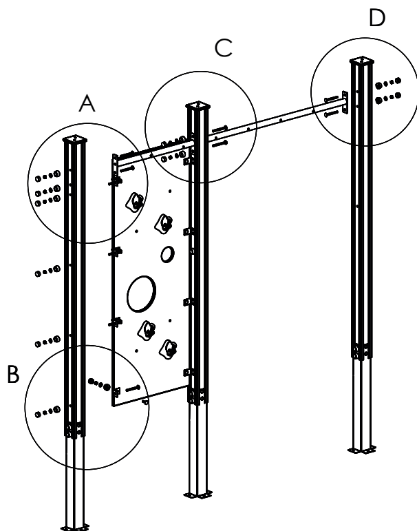
DETAIL A SCALE 1 : 15
