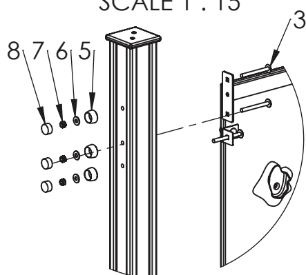
DETAIL F SCALE 1 : 15
