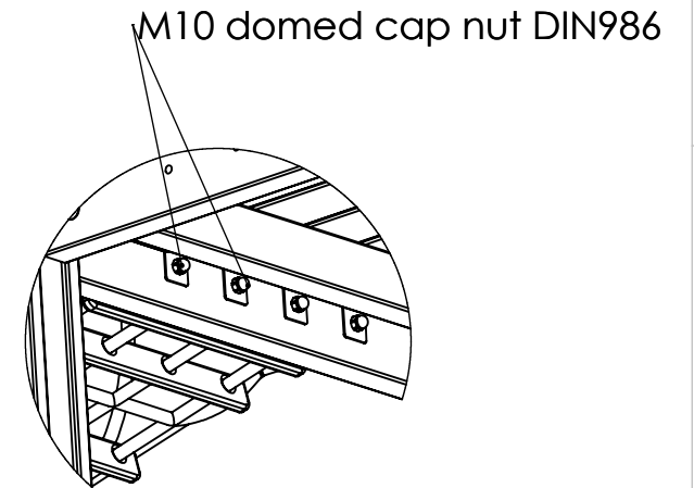
DETAIL H SCALE 1 : 10
