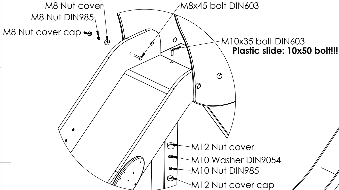
DETAIL E SCALE 1 : 10
