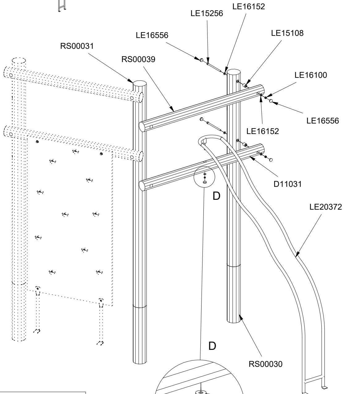
Parts List
