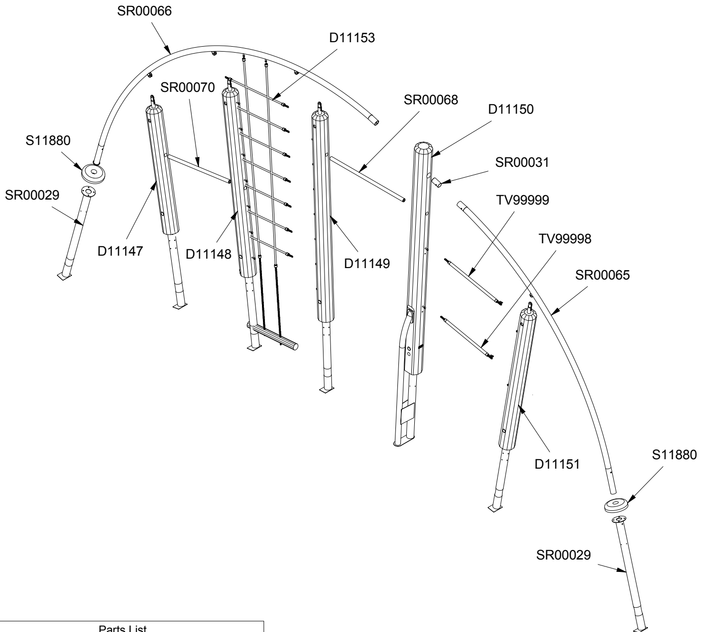
Parts List
