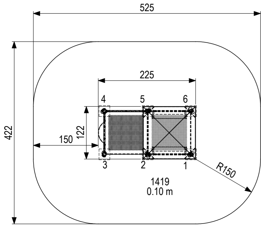
Scale 1:50
