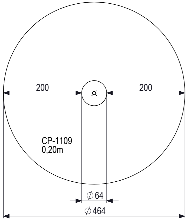
SCALE 1:50
