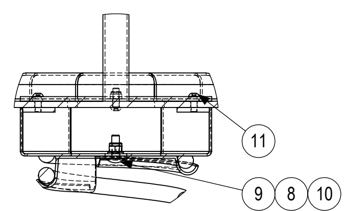
DETAIL B SCALE 1 : 5
