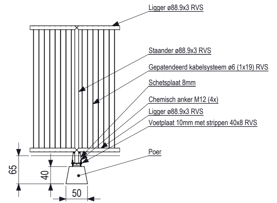
DETAIL A SCALE 1 : 50
